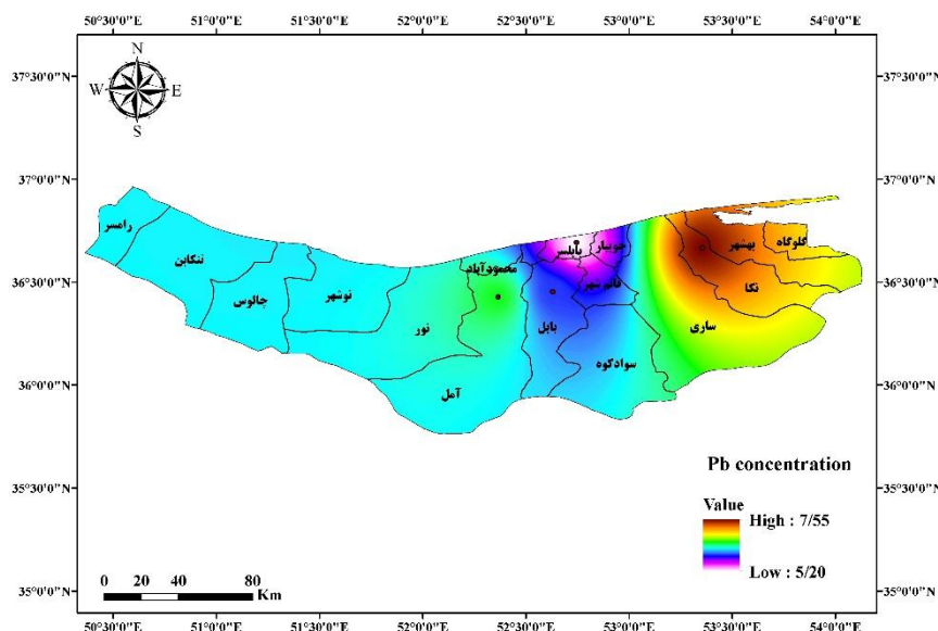
Figure 2. Map of Pb ( \mu\text{g/dl} ) distribution pattern in Mazandaran Province using IDW method.
