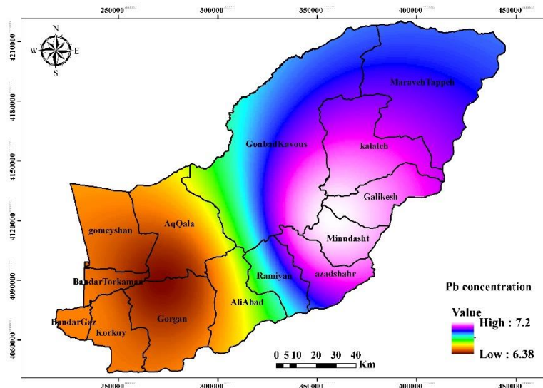
Figure 1. Map of Pb ( \mu\text{g/dl} ) distribution pattern in Golestan Province using IDW method.
