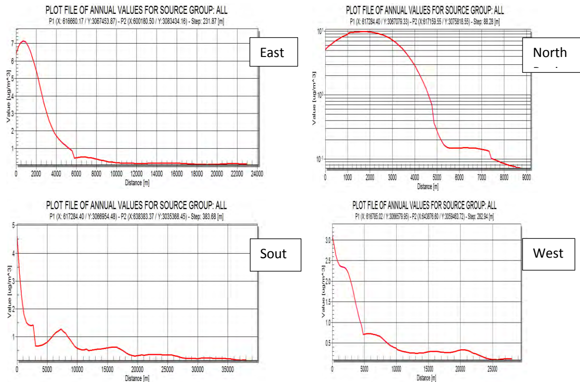
Figure 27. \text{NO}_x emission radius in 4 main directions of the 9 th Refinery of South Pars Gas Complex, Phase 12 of 2021
