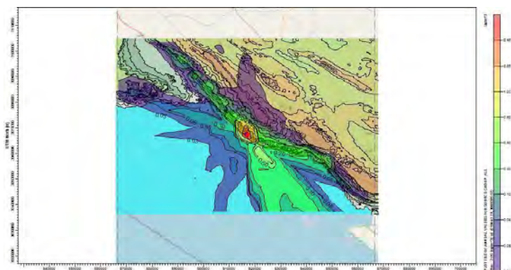
Figure 21. Sulfur dioxide emission of 9 th South Pars Gas Complex, Phase 12 in 2020
