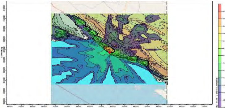
Figure 19. Sulfur dioxide emission of 9 th Refinery of South Pars Gas Complex, Phase 12 in 2020
