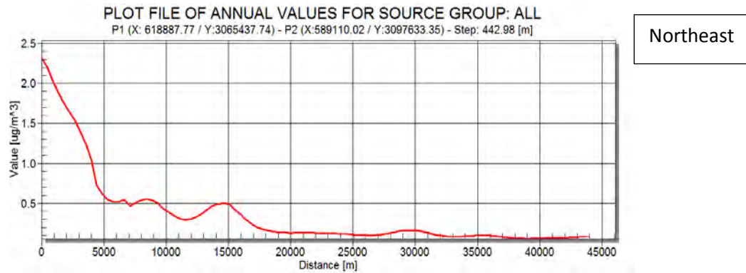
Figure 26. \text{NO}_x emission radius in 4 main directions of the 9 th Refinery of South Pars Gas Complex, Phase 12 in 2020
