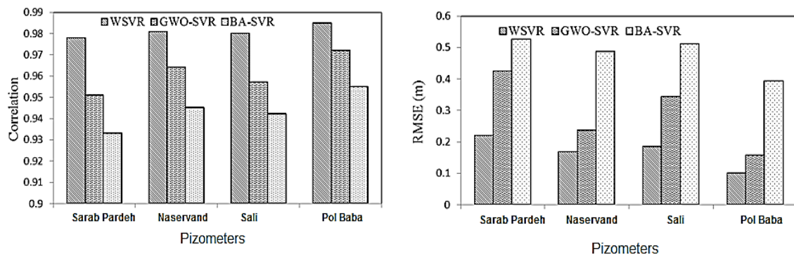
Figure 4. Accuracy and error diagram of the investigated hybrid models
