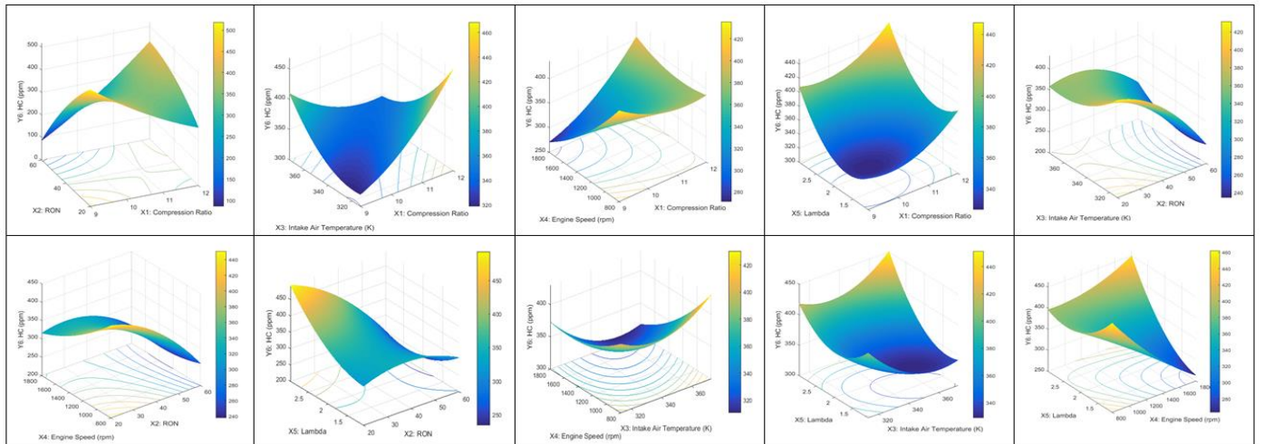
Figure 6. Response surface of HC (ppm)
