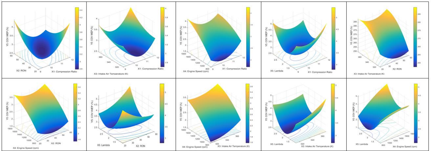
Figure 5. Response surface of COV IMEP (%)
