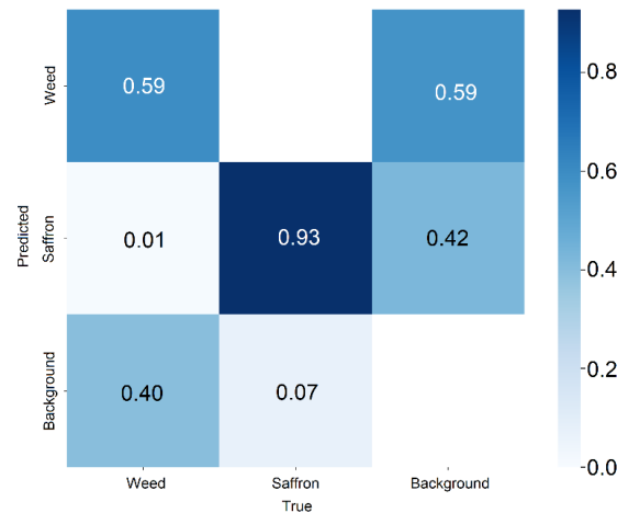
Figure 7. Confusion matrix of the improved YOLOv5s model
