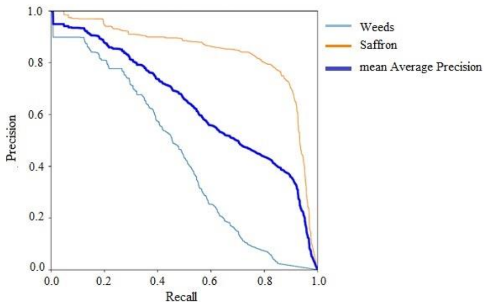
Figure 5. Precision-Recall curve of the improved YOLOv5s model
