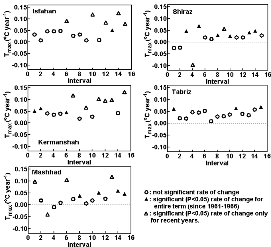
Figure 2. The rate of change in averaged maximum temperature ( T_{\max} ) over 13-days intervals in growing period of chickpea and maize for five locations of Iran. The growing period of two crops overlap over intervals #6 to #8.
