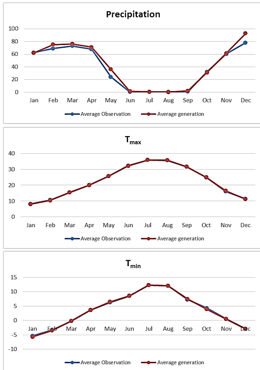
Figure 4. Comparison of observed and modeled values on a monthly scale
