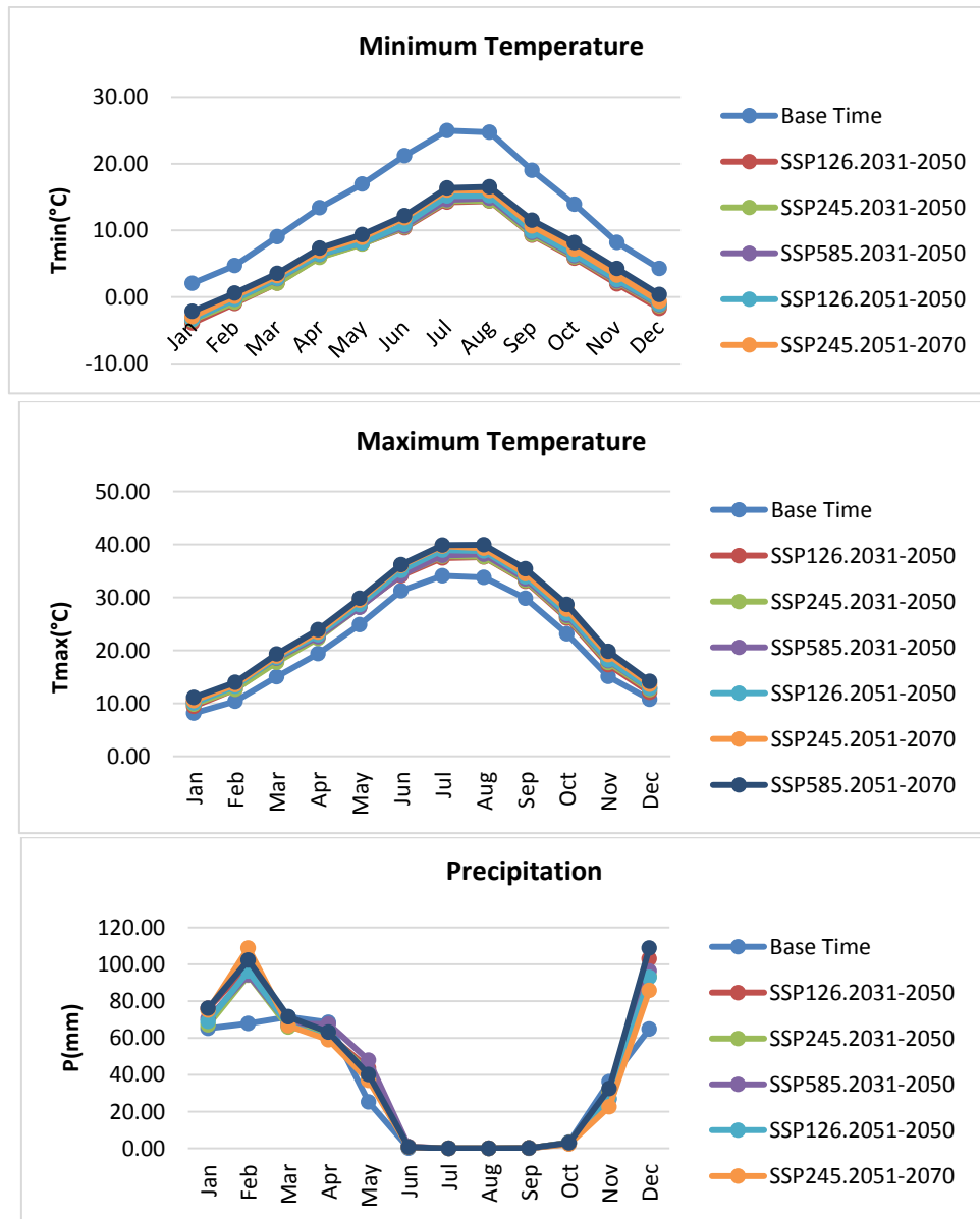
Figure 5. Comparison of monthly fluctuations of meteorological parameters of Al-Shater station in future time periods compared to the base period
