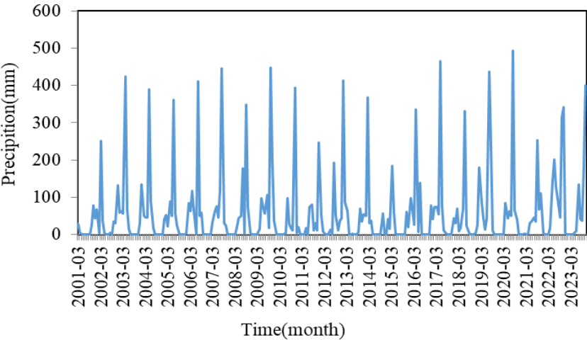
Figure 2. Precipitation trend of the study area
