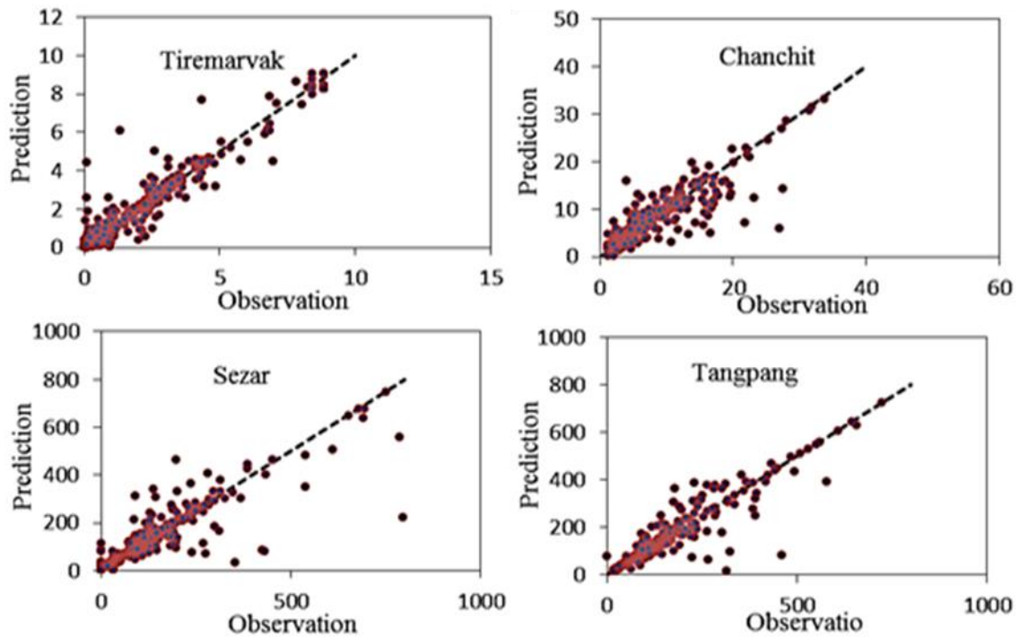
Figure 6. Scatter plot of observed and computed values for the support vector regression-wavelet algorithm model
